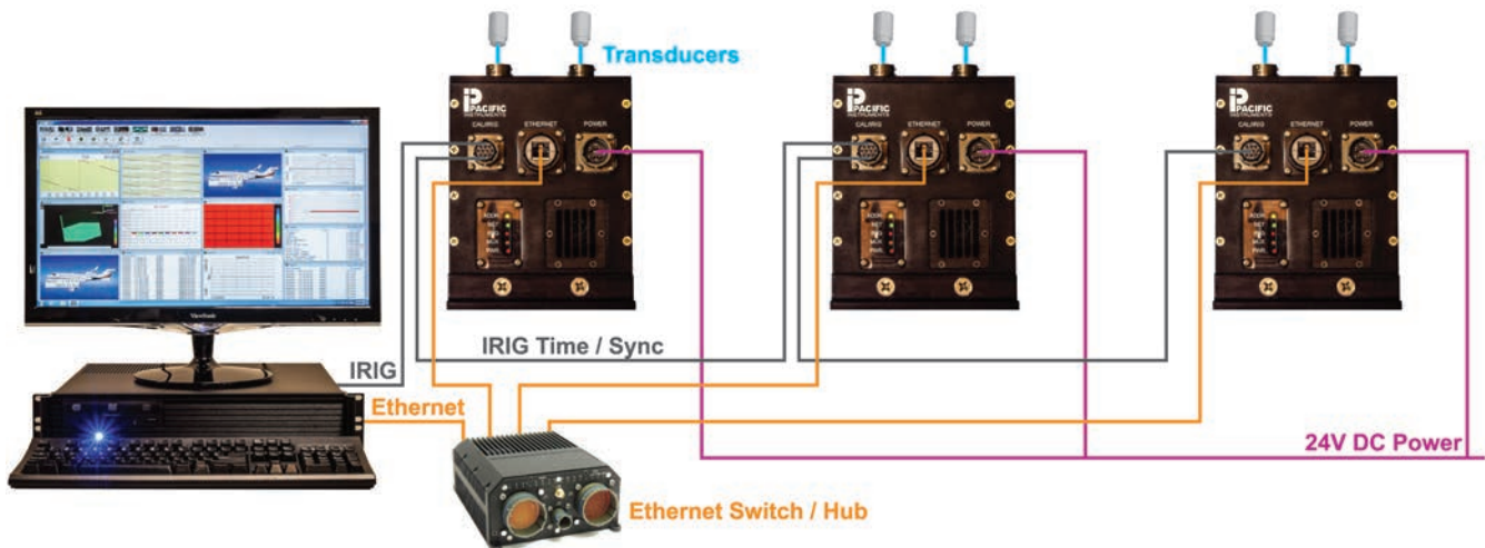
Typical 7300 Installation
